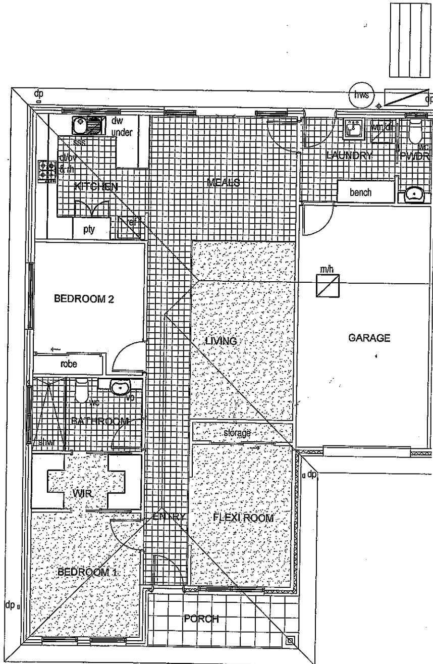
"MILLA" LAYOUT PLAN
